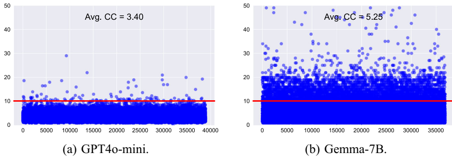
Fig. 3 Comparison of Cyclomatic Complexity between GPT4o-mini and Gemma-7B
