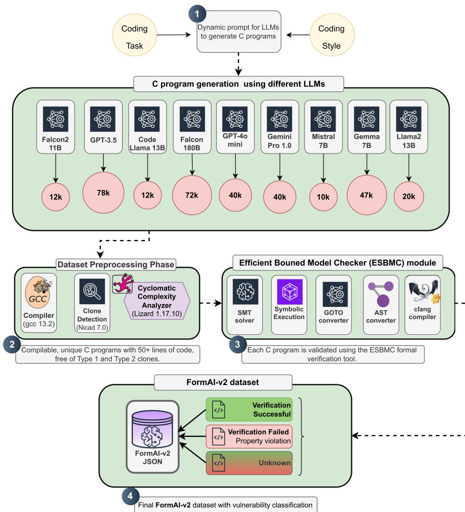
Fig. 2 FormAI-v2 dataset generation Framework using different LLMs
