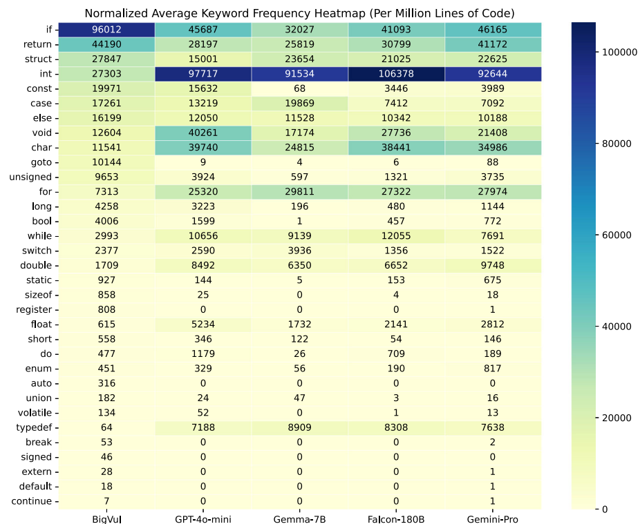
Fig. 4 32 C keyword distribution
